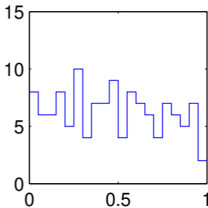
Bandpowers 1–9 \chi^2
