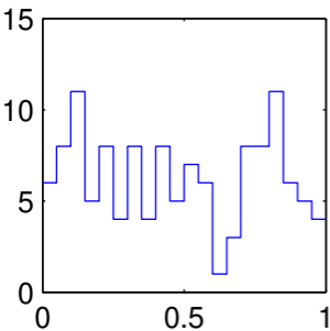
Bandpowers 1–5 \chi^2
