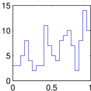
Bandpowers 1–9 \chi
