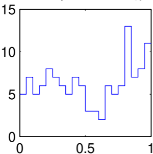
Bandpowers 1–5 \chi
