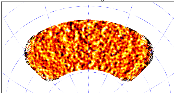
220 GHz Q signal
