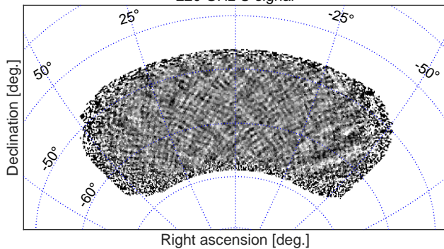
220 GHz U signal
