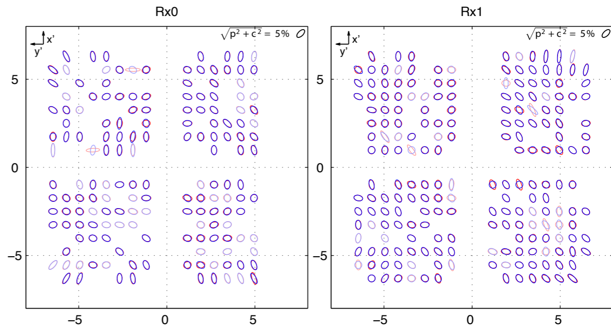
Keck 2013, Ellipticity
