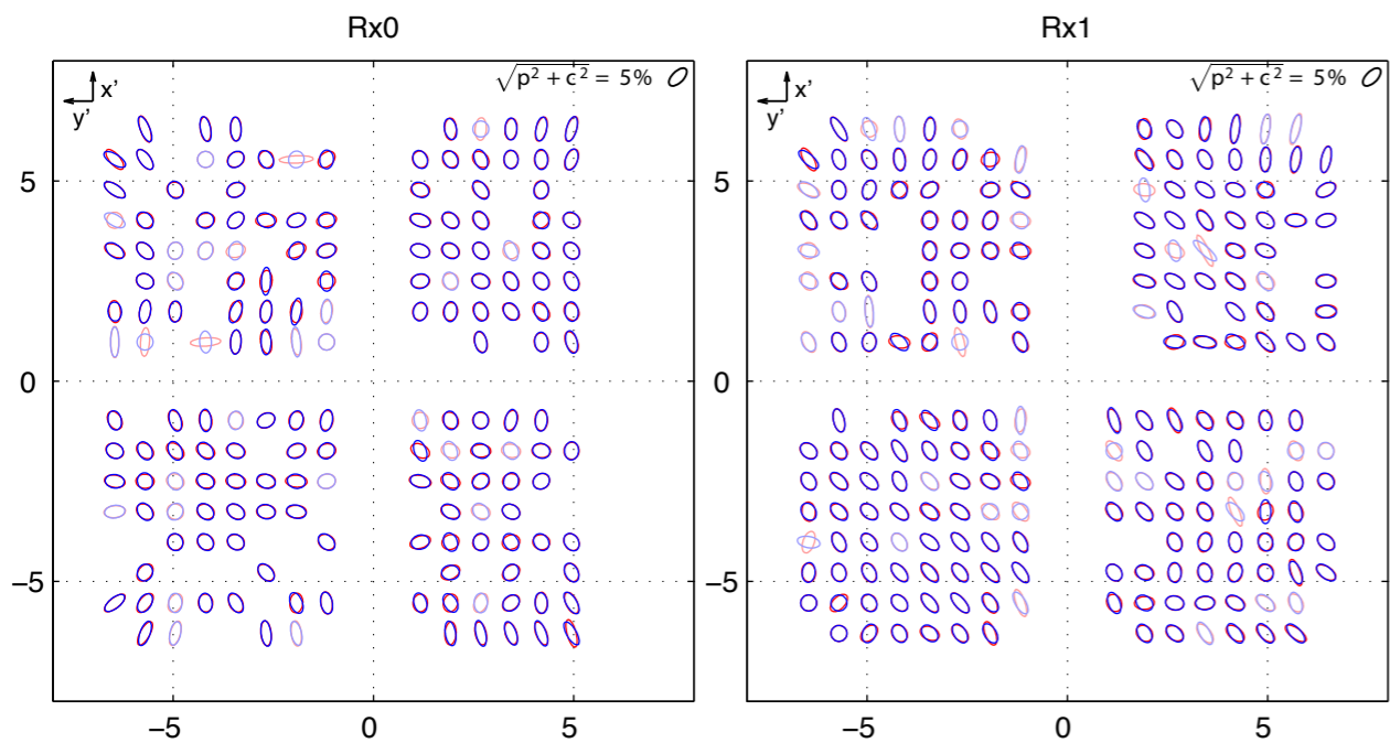
Keck 2012, Ellipticity
